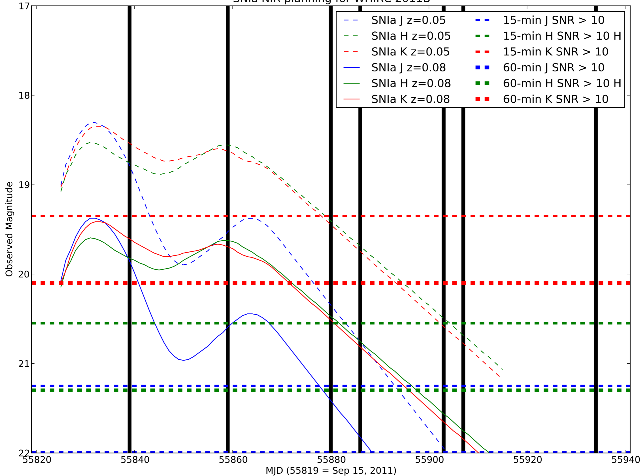
SN Ia NIR planning for WHIRC 2011B
