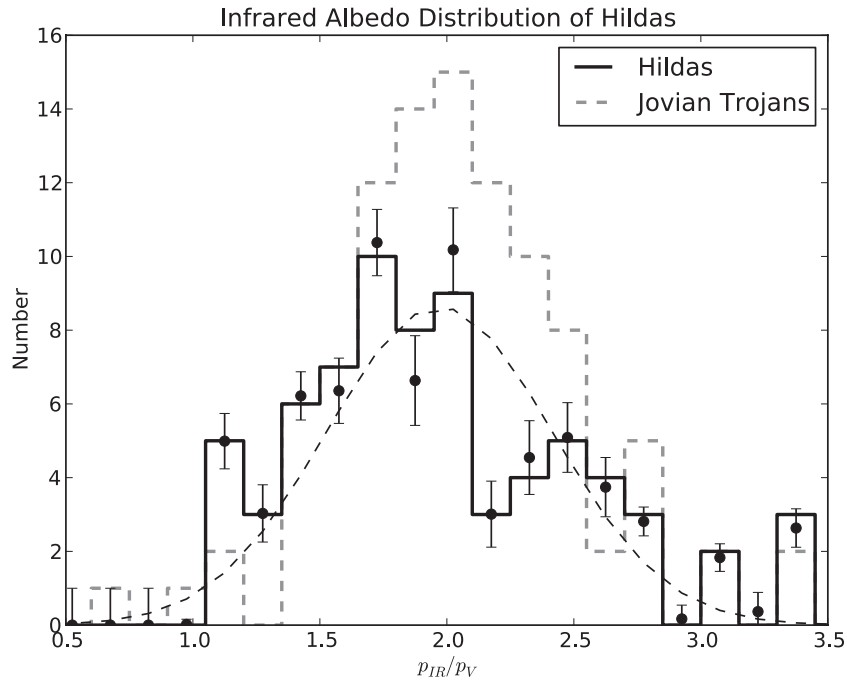
Figure 5. Distribution of the p_{IR}/p_V values based on the 72 objects for which there were observations in either the W1 , W2 , or both bands. The points with associated error bars is the Monte Carlo (MC) error analysis described in the text based on 100 trial runs. The best-fit single Gaussian distribution, which has a mean and standard deviation of 1.9 \pm 0.4 , is shown as a dashed line.
